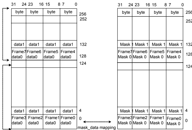
Frame mask definition: only used bit0&bit1 per byte
