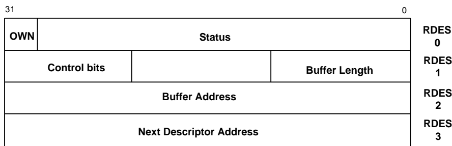
Receive Descriptor Format
